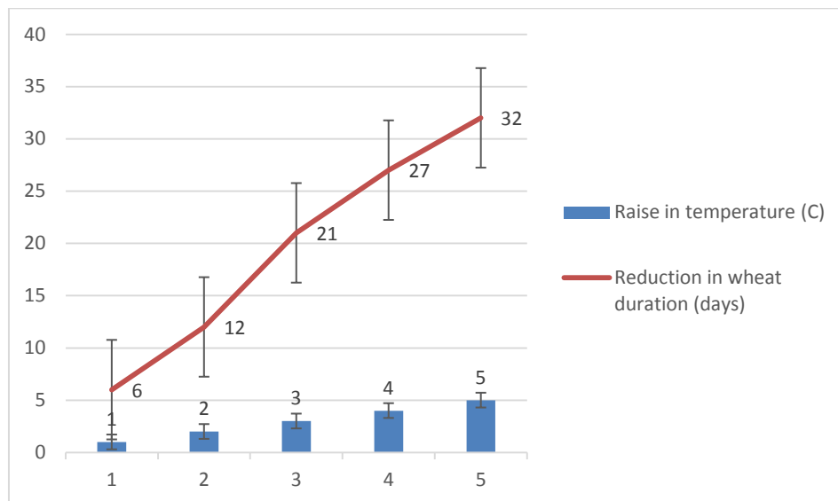
Fig. 2. The consequence of increasing temperature and reduction of the wheat growing duration
