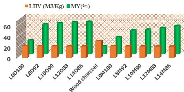
Fig. 5. Evolution of biofuel characteristics with binder content
