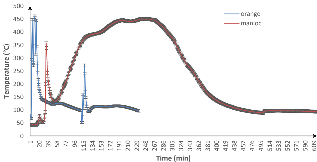
Fig. 3. Evolution of carbonization temperature of Citrus sinensis and Manihot esculenta peels
