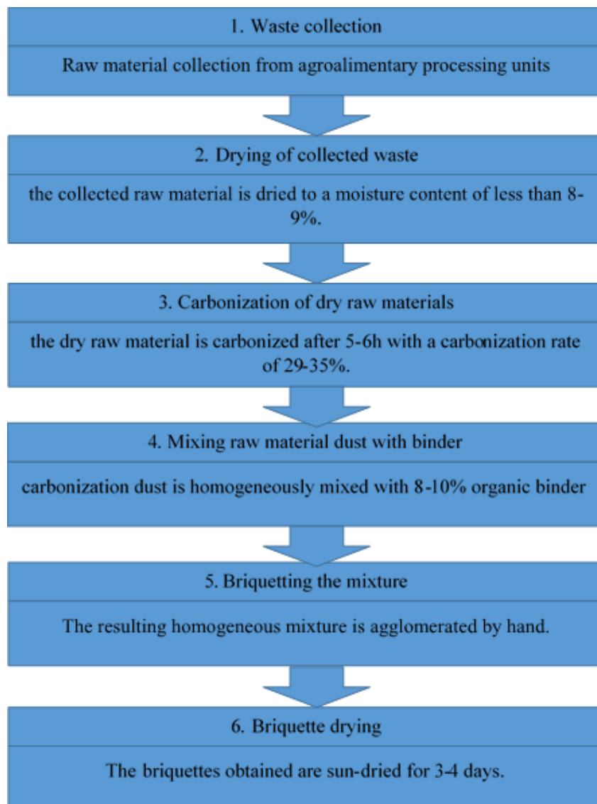
Fig. 2. Biofuel formulation stage
