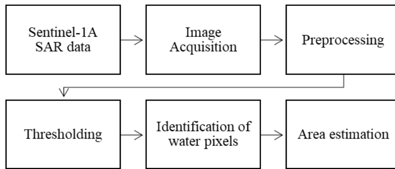
Fig. 2. Methodology
