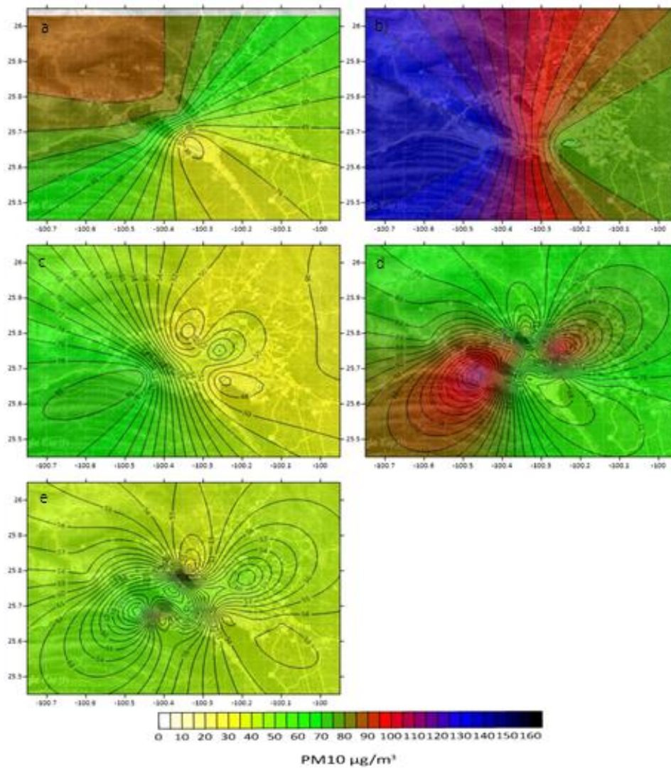
Fig. 7. Temporal space distribution for the highest month of PM 10 (µg/m 3 ) in the MMZ; a) 2000, b) 2005, c) 2010, d) 2014 and e) 2020)
