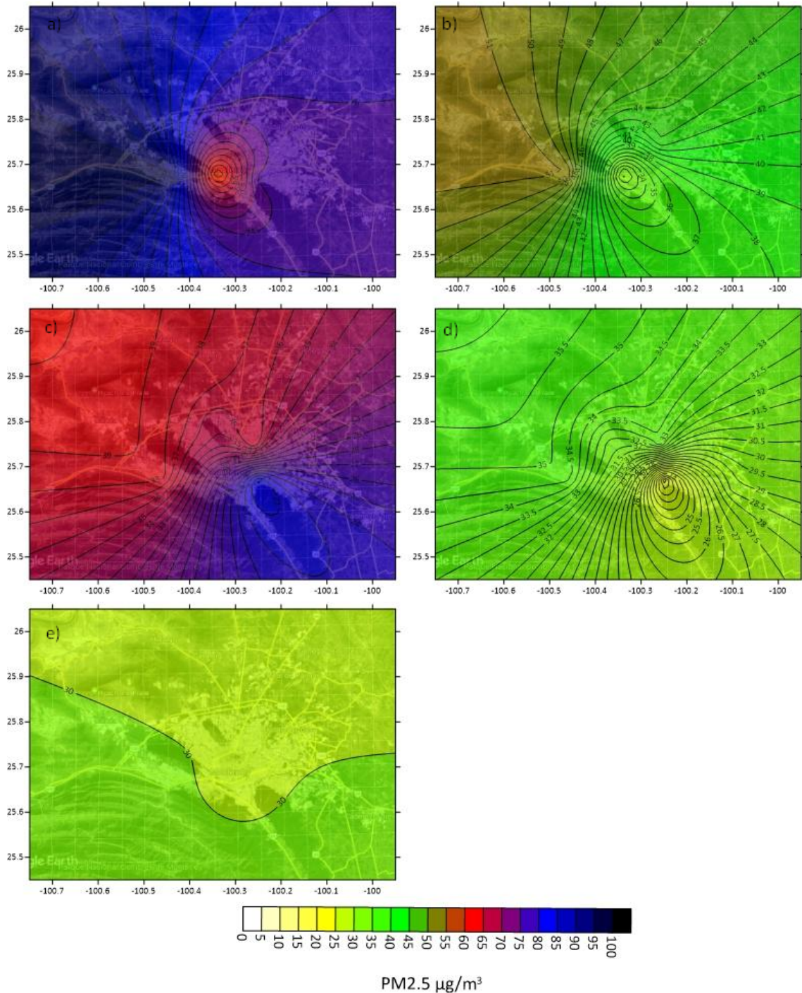
Fig. 10. Temporal space distribution for the highest month of PM 2.5 (µg/m 3 ) in the MMA; a) 2000, b) 2005, c) 2010, d) 2014 and e) 2020)
