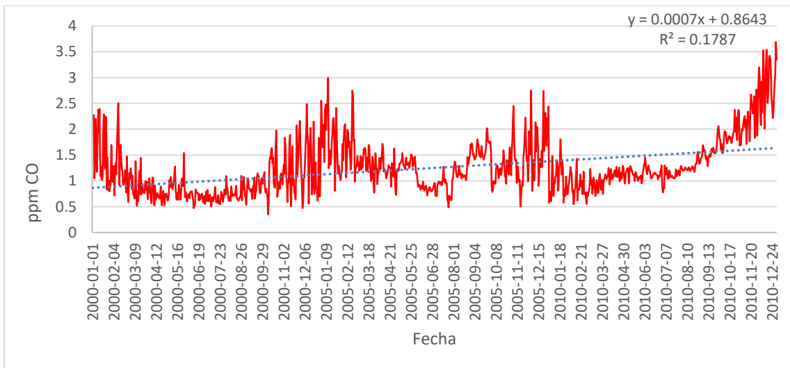
Fig. 20. Daily average CO in ppm in the MMA (2000, 2005, 2010 and 2014)
