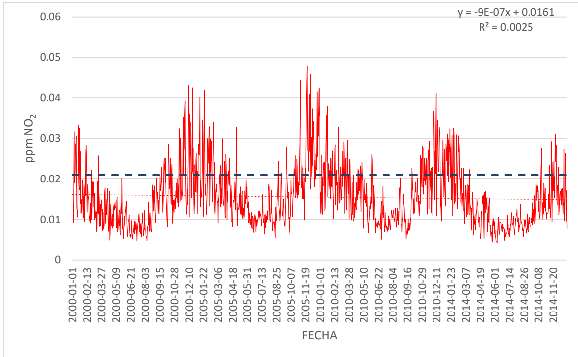
Fig. 17. Daily average of NO 2 in ppm in the MMA (2000, 2005, 2010 and 2014)
