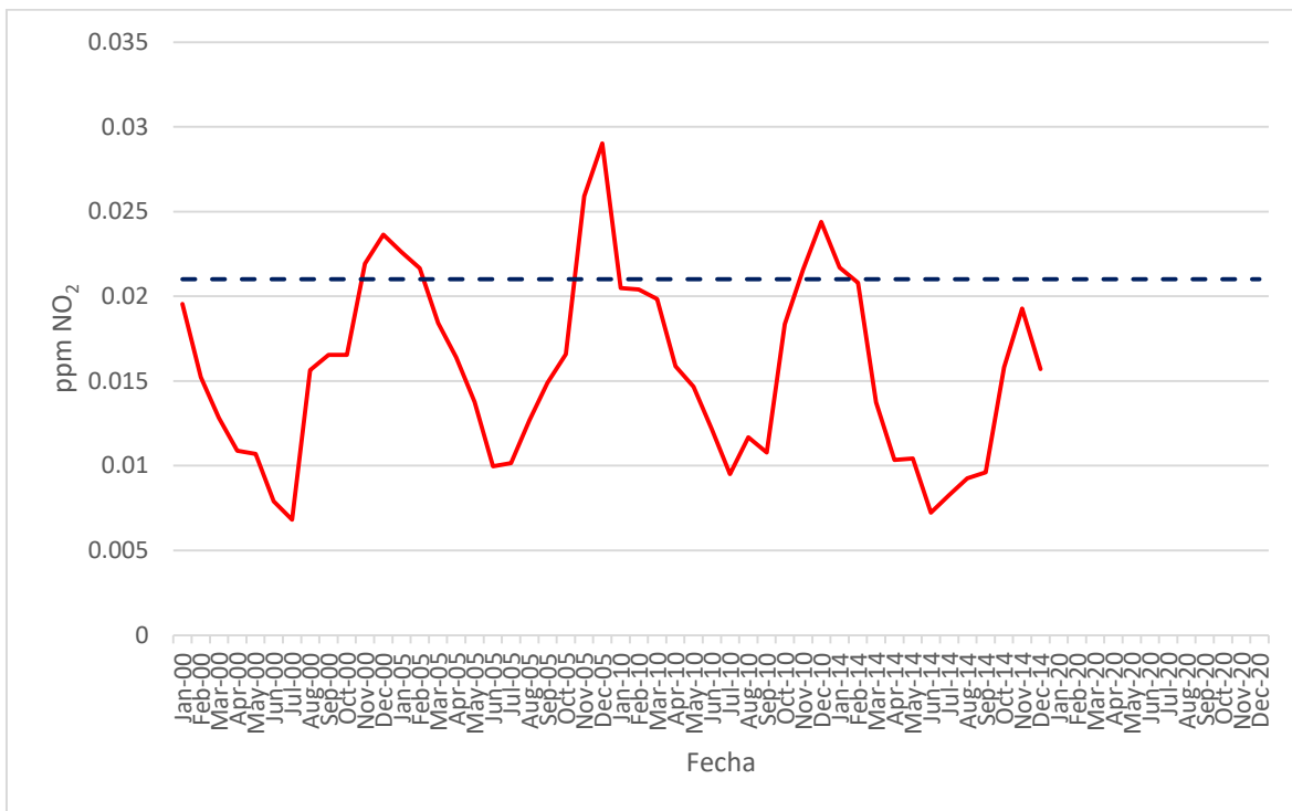
Fig. 18. Monthly average of NO 2 in ppm in the MMA (2000, 2005, 2010 and 2014)
