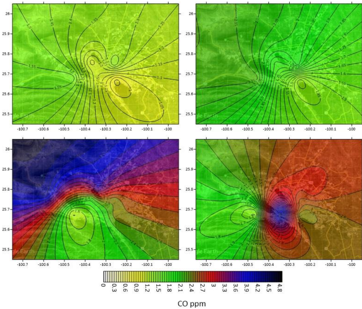
Fig. 22 Temporal space distribution for the highest month of CO (ppm) in the MMA; a) 2000, b) 2005, c) 2010 and d) 2014
