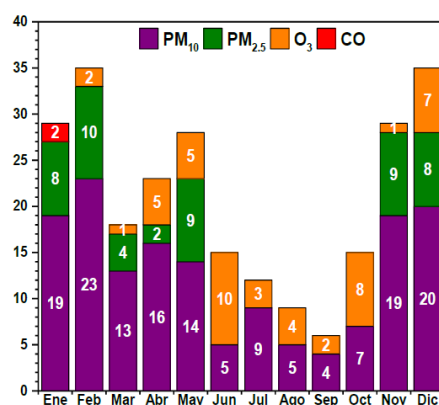
Fig. 4. Days out of Environmental Health NOMs by pollutant in the MMA in 2019
