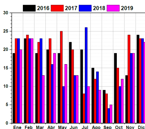
Fig. 3. Days out of Environmental Health NOMs in the MMA (2016-2019)
