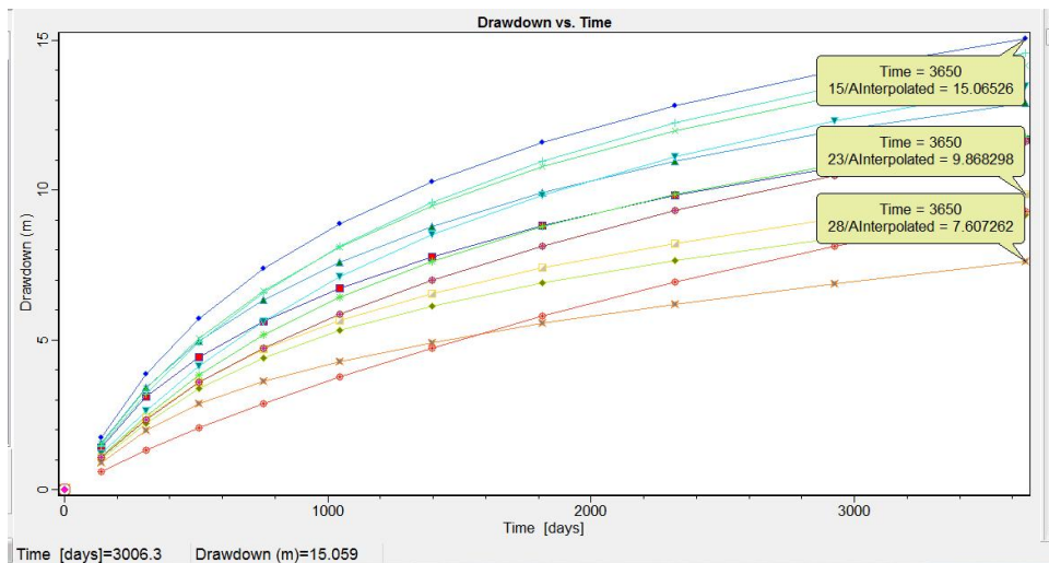
Fig. 8. The expected drawdown in wells versus time
