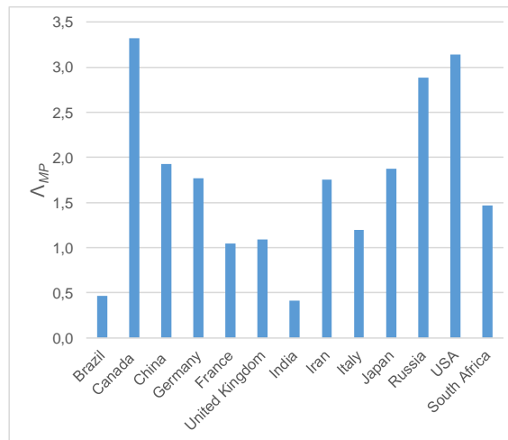
Fig. 1. \Lambda_{MP} indicator for carbon dioxide emissions of a selected group of countries. For the calculation data from Refs. [5 and 6] are used
