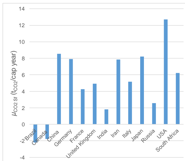
Fig. 3. Carbon dioxide emission indicator for a selected group of countries, based on data from the Refs. [5, 6 and 7]
