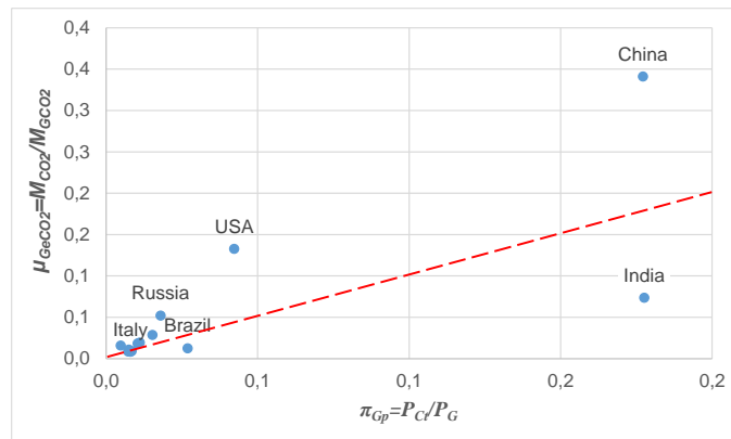
Fig. 2. Considered countries in the diagram: "Share in global population - share in global carbon dioxide emissions", based on data from Refs. [5 and 6]
