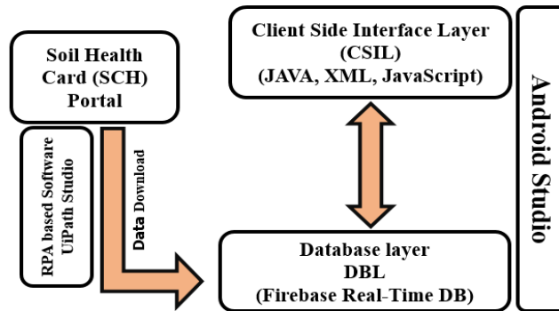
Fig. 3. Application architecture of SoilNutro
