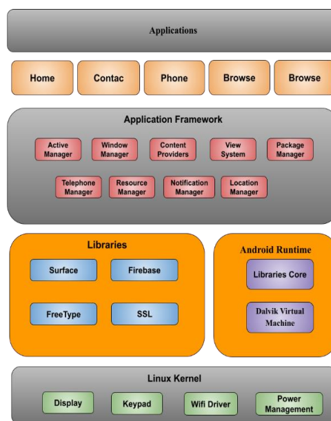
Fig. 2. Application framework of android
