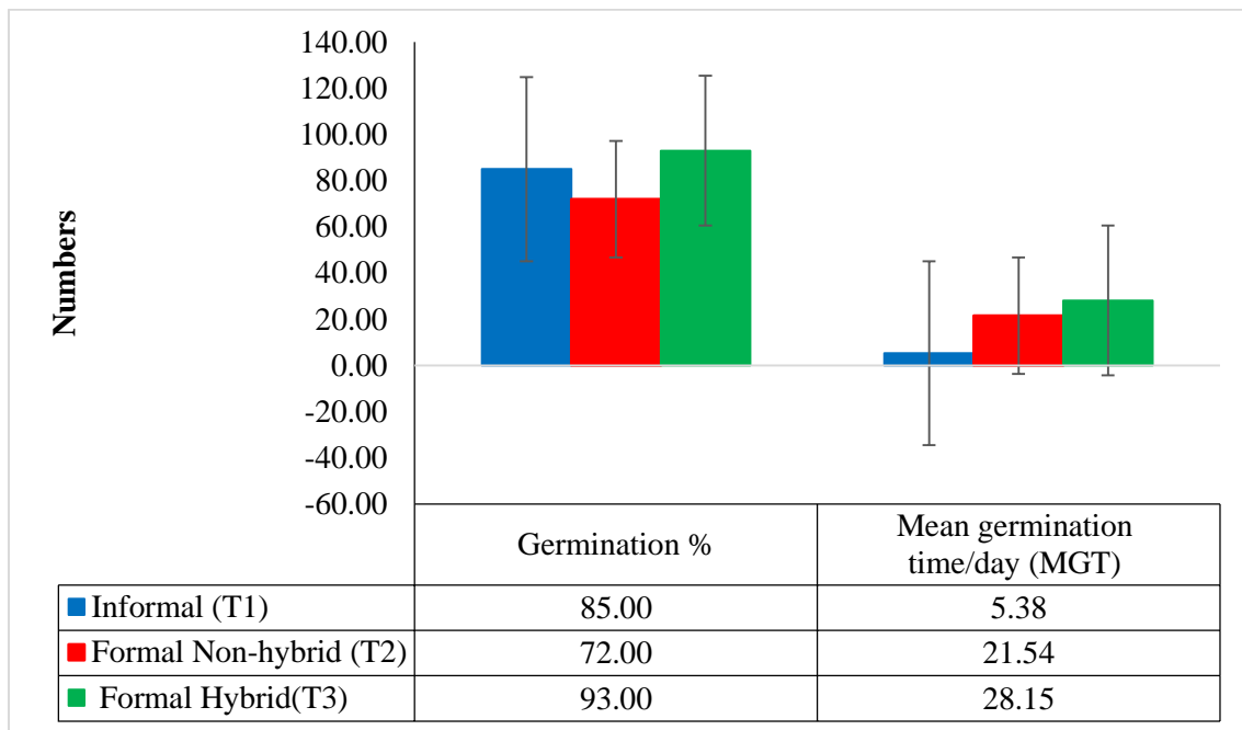
Fig. 2. Mean percentage germination and mean daily germination
