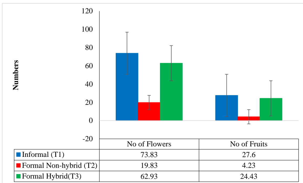
Fig. 3. The mean number of flowers and fruits of different tomato seed systems
