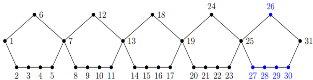
Fig. 3. C_{7,2}^5 with the modified cyclic snake labelling F(x)
