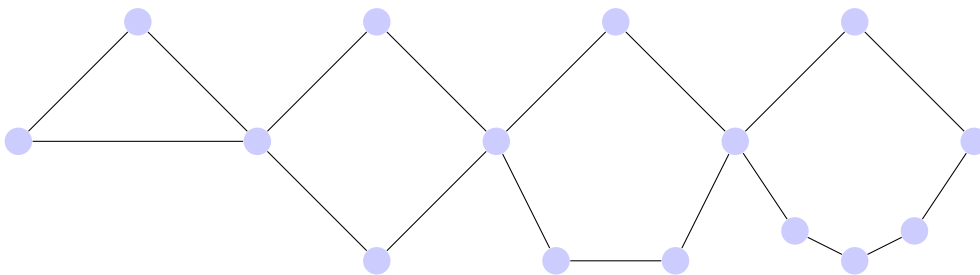
Fig. 4. The snake graph with different k values
