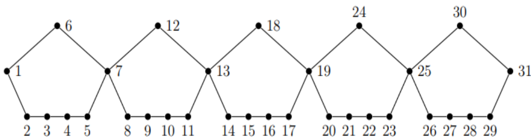
Fig. 2. C_{7,2}^5 with the cyclic snake labelling f(x)
