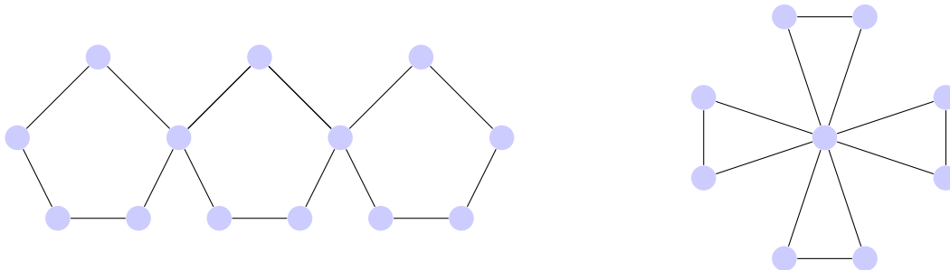
Fig. 1. Two examples of snake graphs; C_{5,2}^3 and C_{3,0}^4 respectively
