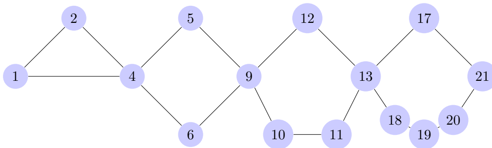
Fig. 5. The labeled snake graph with different k values
