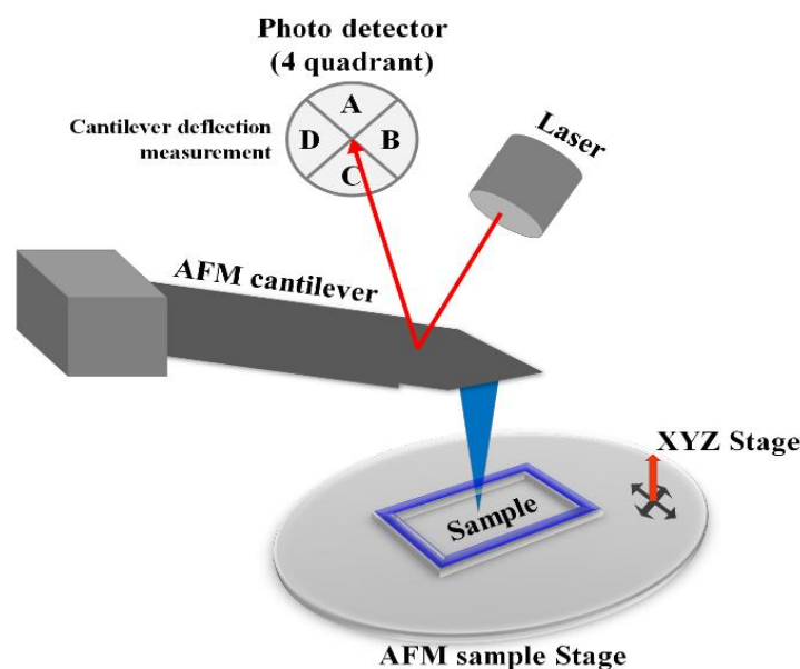
Fig. 2. Schematic diagram of AFM
