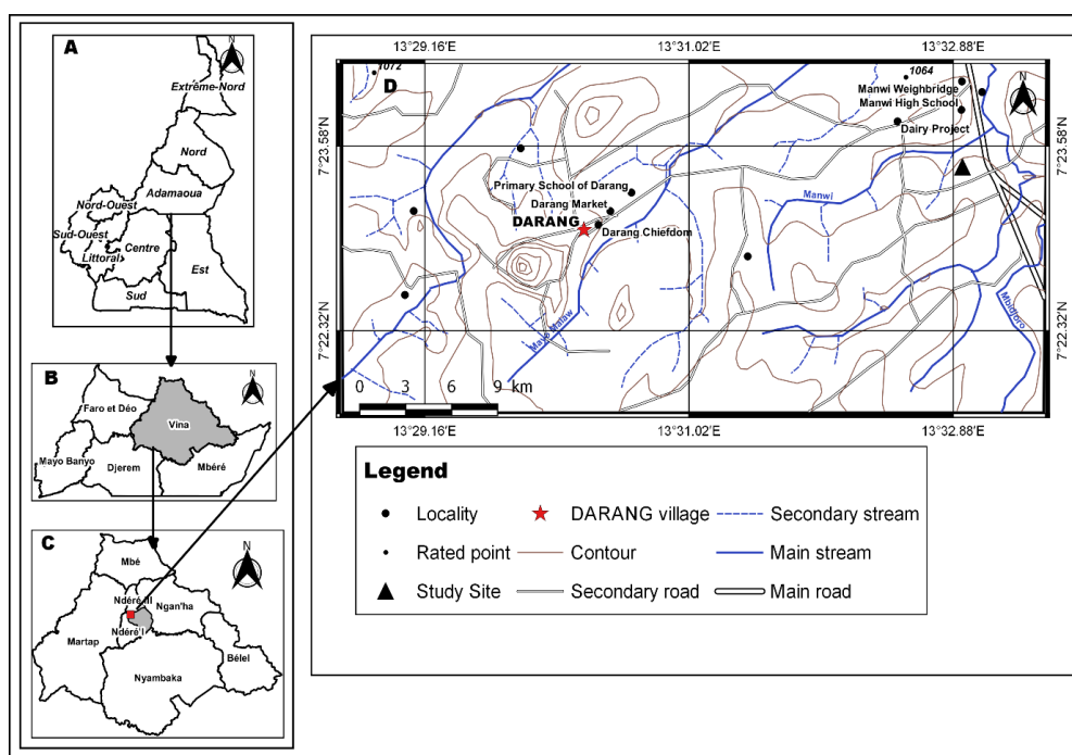
Fig. 1. Localization of study area (obtained from SOGEFI 2019 database coupled with topographic map of Ngaoundéré at 1:200,000, associated with field data)
