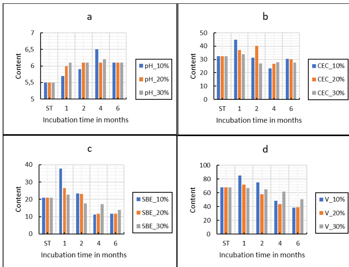
Fig. 2. Variation of: a) pH; b) Cationic Exchange Capacity; c) Sum of Exchangeable Bases and d) saturation rate per treatment
